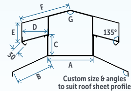
ROLL TYPE RIDGE
